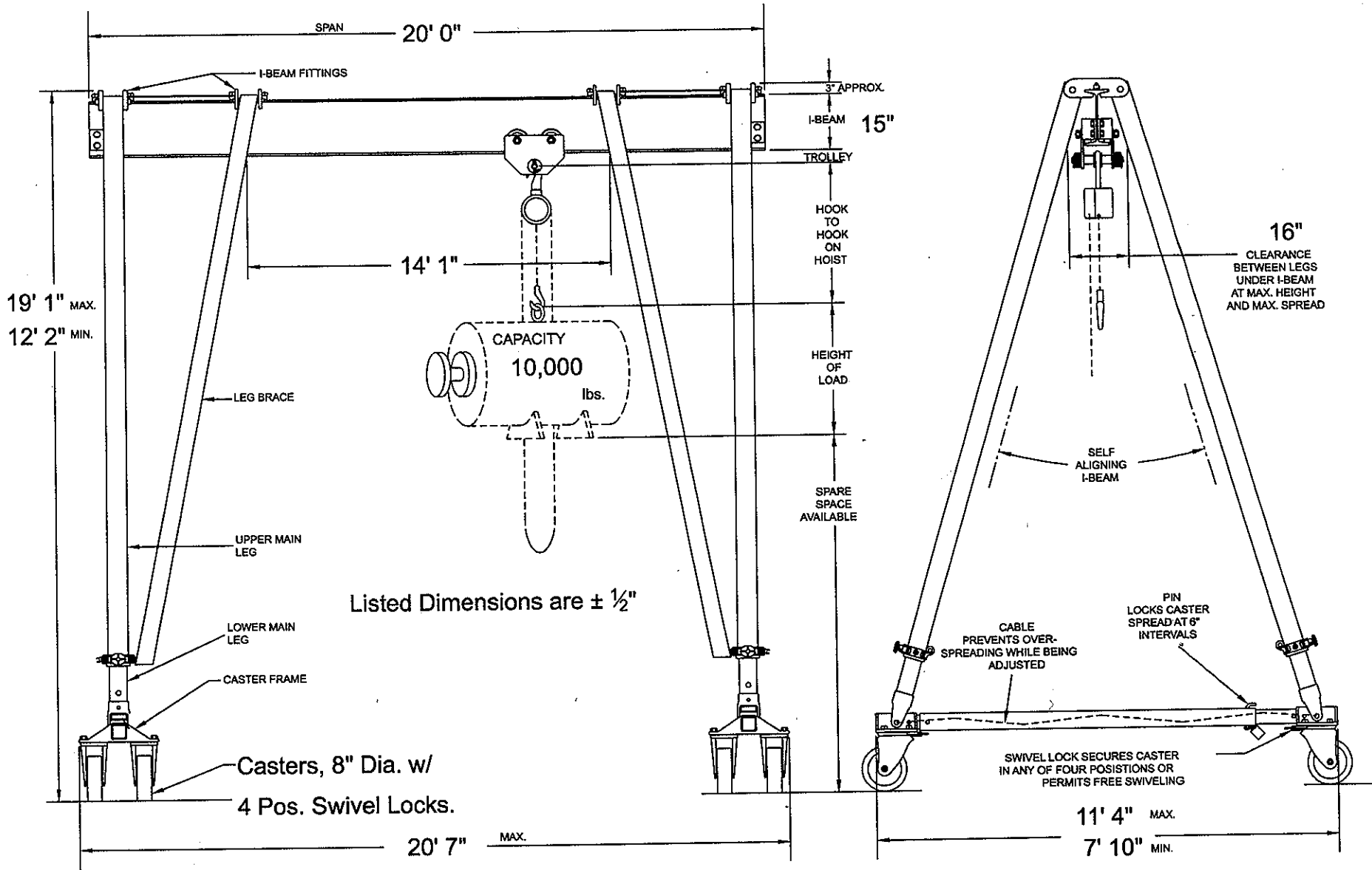
Steel End Frames with Steel I-Beam
