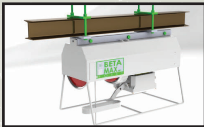
FIXED I-BEAM
