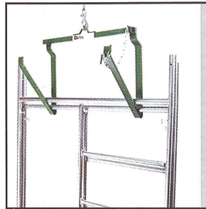
SCAFFOLD FRAME FORK 600 lb. capacity 36 1/4" L x 15" W x 25" H Holds 10 scaffold frames
