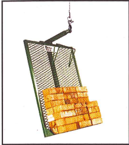
BRICK FORK 400 lb. capacity 29 1/4" L x 7 1/2" W x 37 1/2" H Max. brick size: 2 1/2 x 3 x 8
