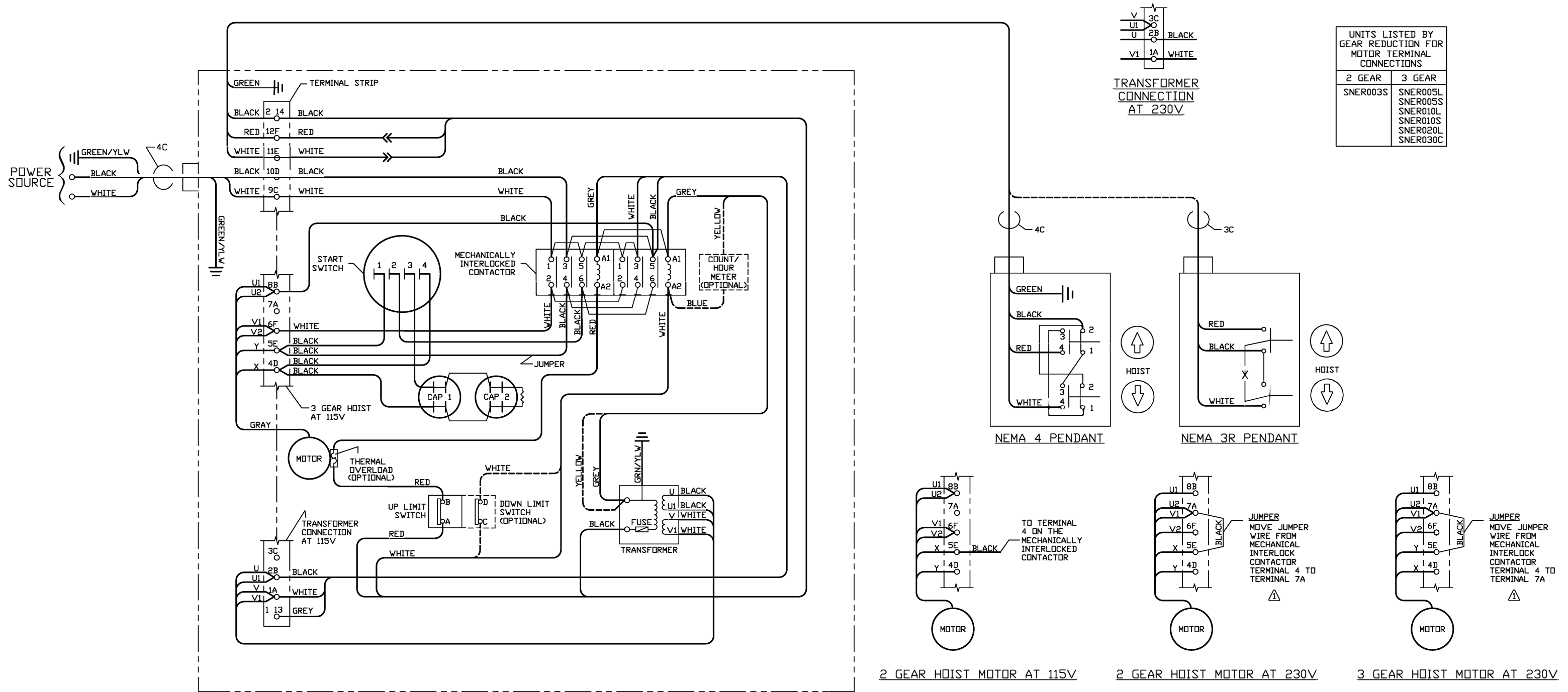
ELECTRIC CHAIN HOIST
